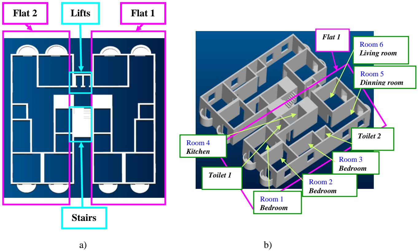
Figure 1. The top view of one floor of the selected residential building (a) and 3D model of one selected flat of the selected building (b)
